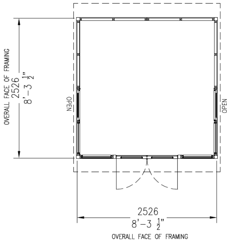
PLAN VIEW
