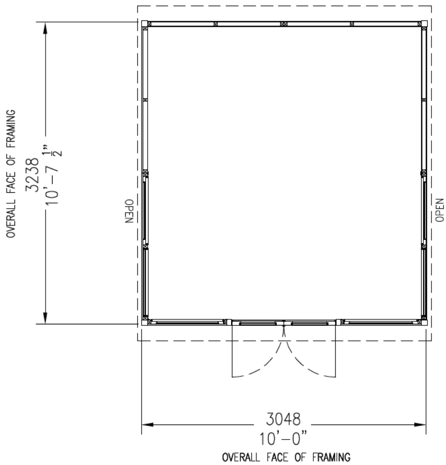
PLAN VIEW
